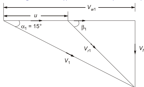
Inlet Velocity Triangle
