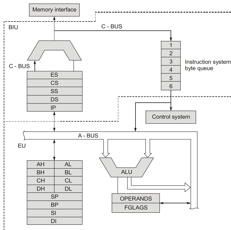
Functional block diagram of 8086
